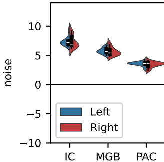
D residuals
