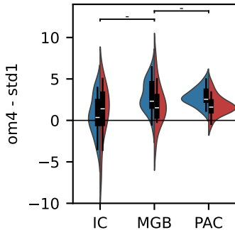
B omissions
