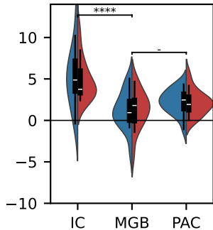
A adaptation
