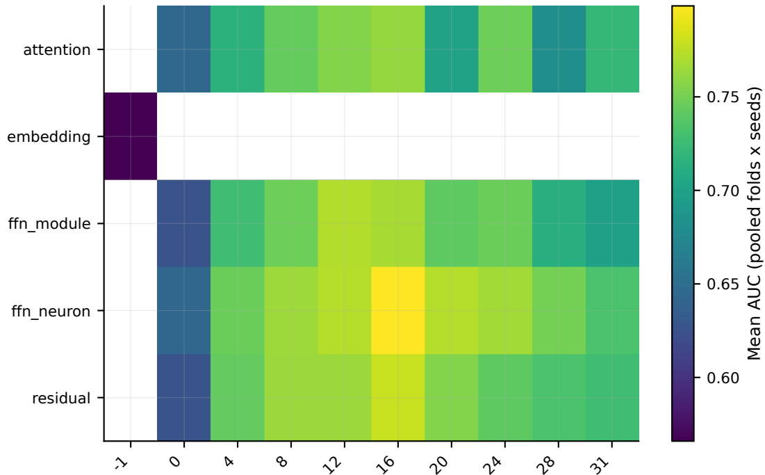
coqa (posthoc) - Full Representation AUC
