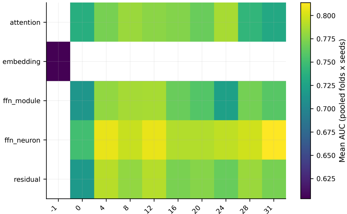
gsm8k (posthoc) - Full Representation AUC
