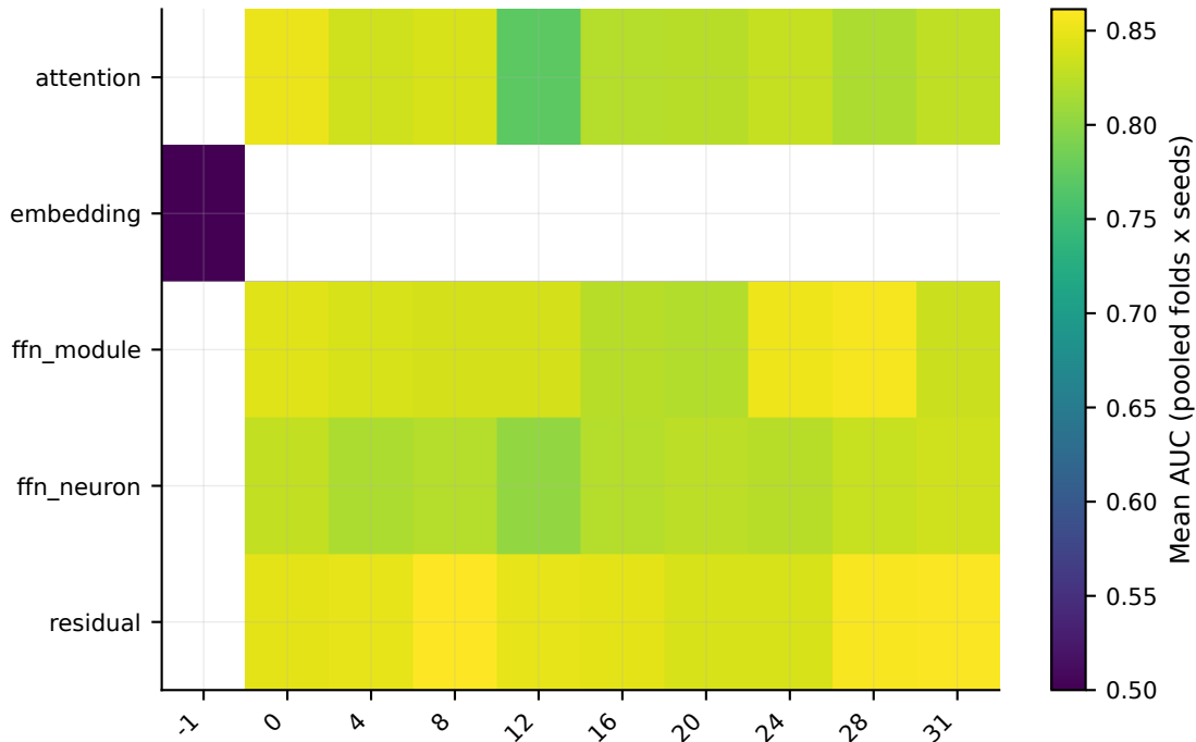
medquad (pregen) - Full Representation AUC
