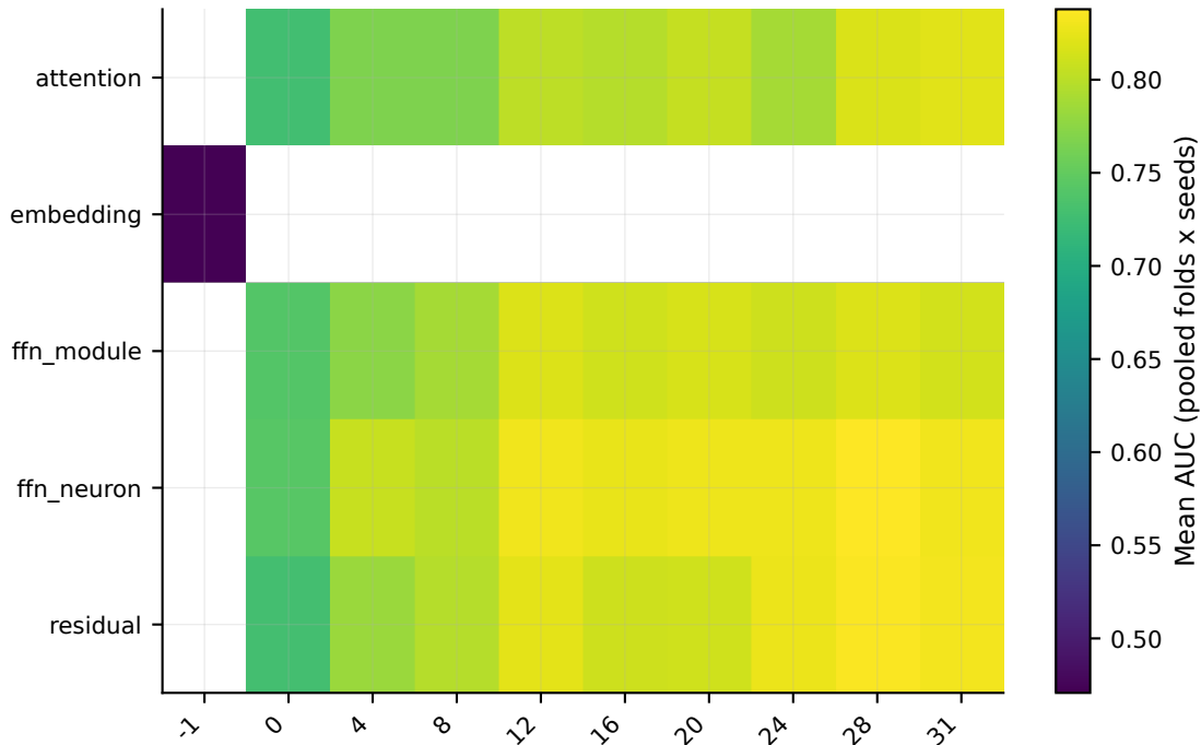
triviaqa (posthoc) - Full Representation AUC
