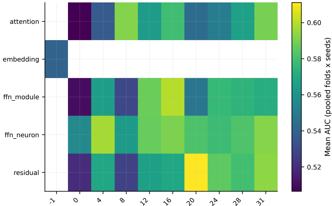
truthfulqa (posthoc) - Full Representation AUC
