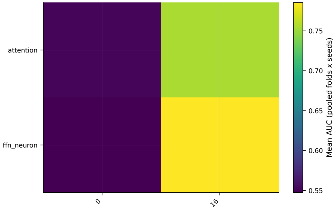
triviaqa (pregen) - Full Representation AUC
