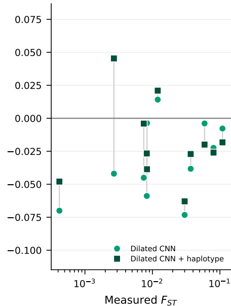
Network - best released tool
