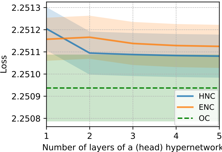
Test loss vs number of layers
