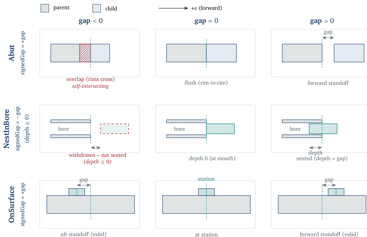
Figure 4. Meaning of StationLink::gap for each SeatKind , with forward ( +z = forward) to the right; gray is the parent, colour the child. Abut (top): the gap is a signed forward standoff — flush at \text{gap} = 0 , an open seam for \text{gap} > 0 , and a self-intersecting placement (the child driven into the part it mates) for \text{gap} < 0 ; the child is drawn seated forward of its parent so a positive gap reads as separation. NestInBore (middle): the gap is a non-negative insertion depth driving the child aft into the parent bore ( \text{signedGap} = -\text{gap} ) — depth 0 rests the child at the mouth, a positive depth nests it, and a negative value withdraws it from the bore (not seated). OnSurface (bottom): the gap is an axial standoff along the parent wall, valid in either direction (aft for \text{gap} < 0 , forward for \text{gap} > 0 ). In every case the resolver computes \text{childOriginZ} = \text{p.z} + \text{signedGap} - \text{c.z} .
