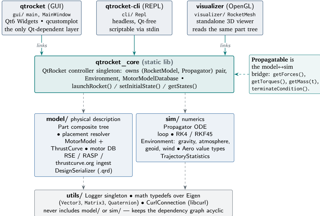
Figure 1. The shipped system: three executables over one Qt-free core. Every edge points strictly downward — front ends link qtrocket_core , the core links model/sim/utils , and utils links only third-party math and networking. The Propagatable interface (right) is the single seam through which the simulation loop sees the rocket model.
