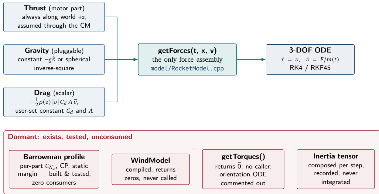
Figure 3. The flight-physics force path at commit 20eca72. Three terms — world-vertical thrust, pluggable gravity, and a single quadratic drag law — are assembled by getForces() and integrated as three linear degrees of freedom. The red-edged layer below is built and tested but has no production caller.
