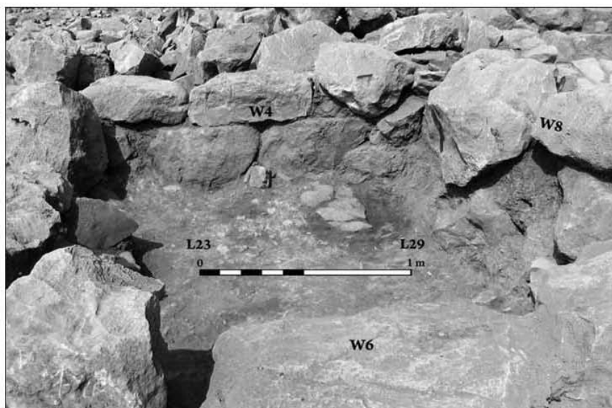
Fig. D6. L23 and baking installation L29, view to the north-west.
