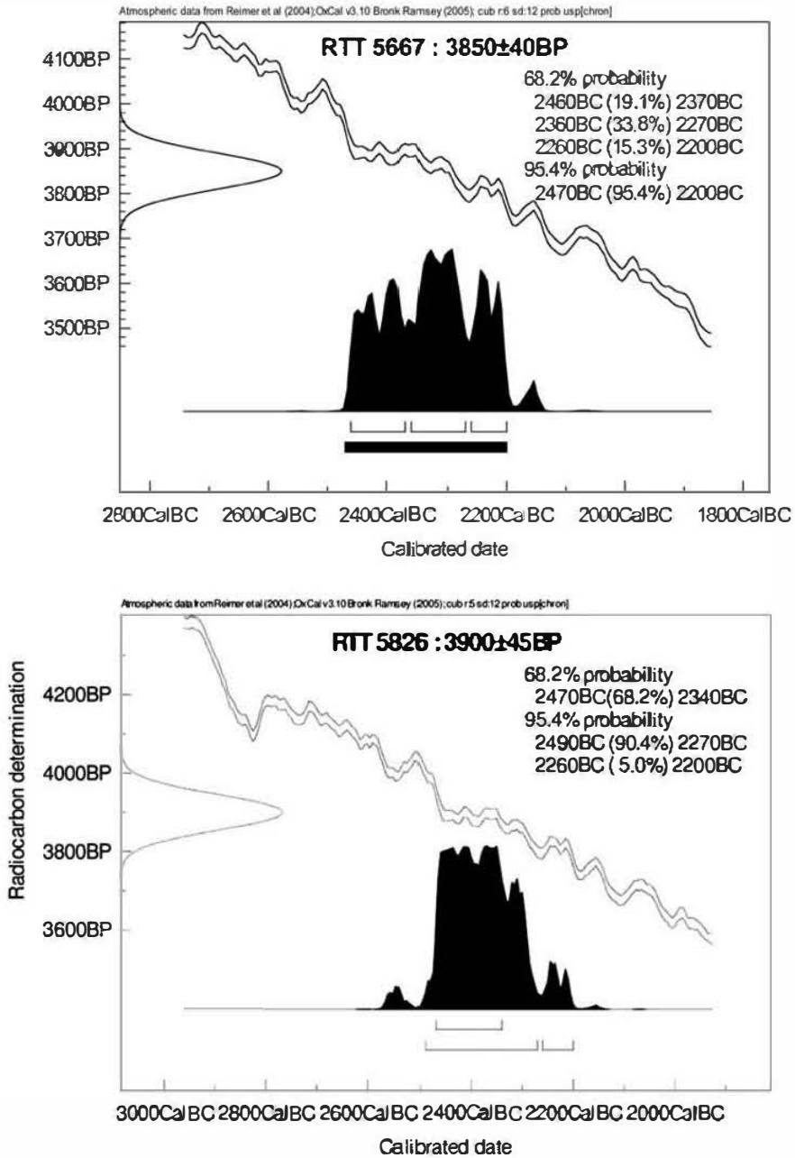
Fig. D16. Radiocarbon date graphs from E.P. -167.
