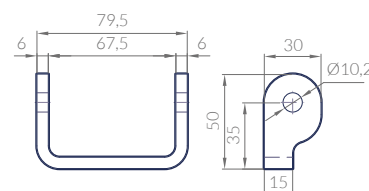
SOPORTE U 15 SBT1MC PARA BISAGRA TRASERA HINGE BRACKET U 15 BOCK IN U-FORM 15 CHAPE U 15
