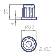
CASQUILLO CBT1MA PALA BISAGRA TRASERA
