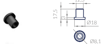
CASQUILLO CBL1MA PARA BISAGRA LATERAL BUSH | KUNSTOFFBUCHSE | DOUILLE
