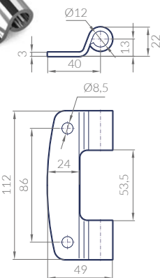
SOPORTE 180 SBL1MC PARA BISAGRA LATERAL HINGE BRACKET 180 BOCK 180 CHAPE 180
