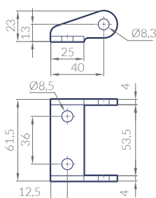
SOPORTE U 25 SBL1MA PARA BISAGRA LATERAL HINGE BRACKET U 25 BOCK IN U-FORM 25 CHAPE U 25
