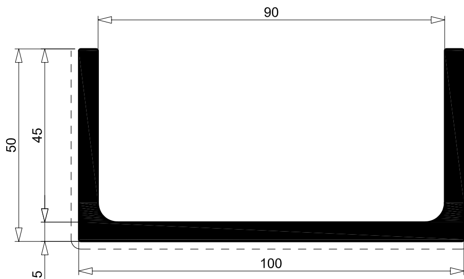
B 1002 2.562 Kg/m sup. in vista 199 mm per. esterno 384 mm
