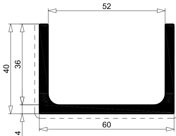
B 1001 1.452 Kg/m sup. in vista 139 mm per. esterno 266 mm
