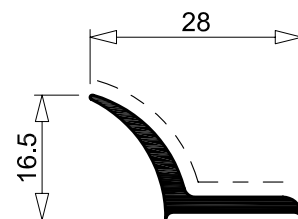
I 35 0.189 Kg/m sup. in vista 32 mm per. esterno 76 mm
