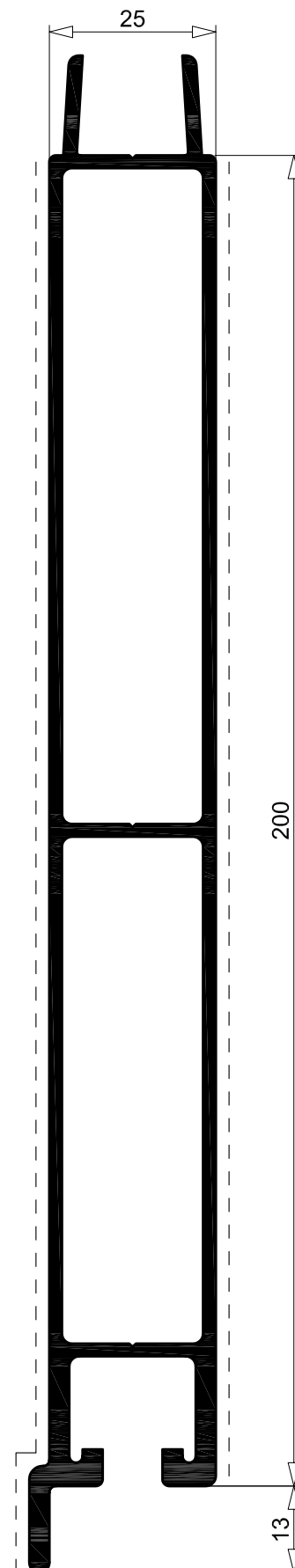
R 3771 2.915 Kg/m sup. in vista 413 mm per. esterno 600 mm
