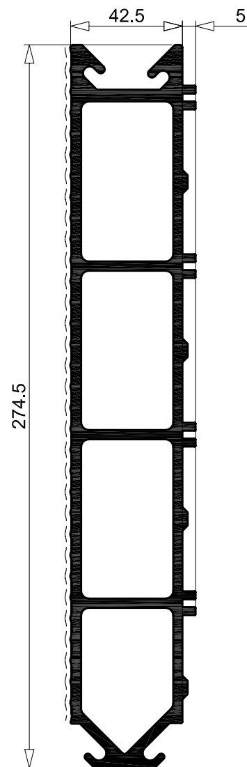
R 10631 8.065 Kg/m sup. in vista 260 mm per. esterno 795 mm
