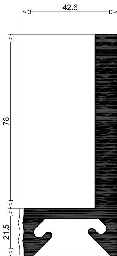
I 7479 3.308 Kg/m sup. in vista 22 mm per. esterno 336 mm
