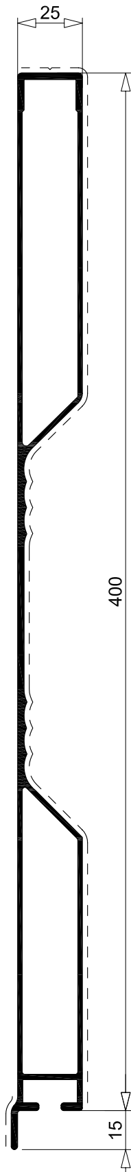
R 3367 4.209 Kg/m sup. in vista 449 mm per. esterno 947 mm
