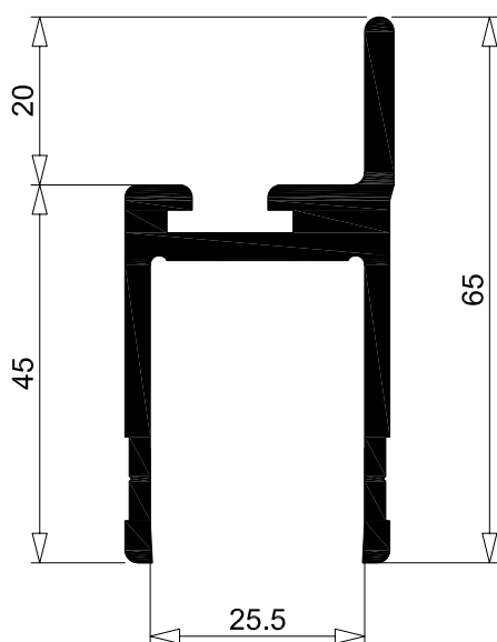
B 331 1.350 Kg/m sup. in vista X mm per. esterno X mm
