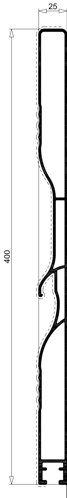
R 12415 4.433 Kg/m sup. in vista 580 mm per. esterno 995 mm
