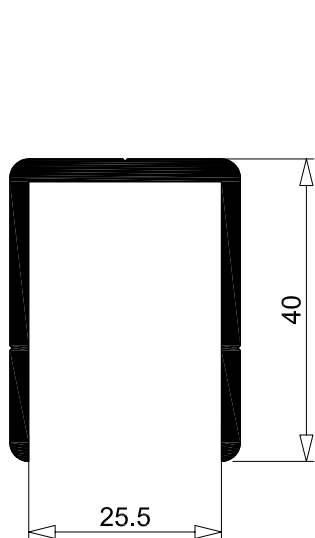
B 326 0.729 Kg/m sup. in vista X mm per. esterno X mm
