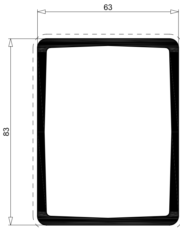
R 3993 2.598 Kg/m sup. in vista 285 mm per. esterno 285 mm
