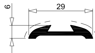
I 85 0.208 Kg/m sup. in vista 24 mm per. esterno 74 mm
