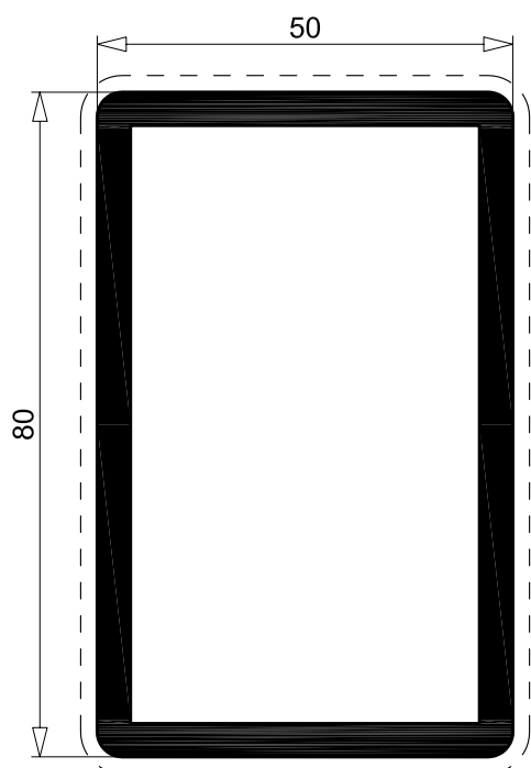
R 5816 2.614 Kg/m sup. in vista 255 mm per. esterno 255 mm
