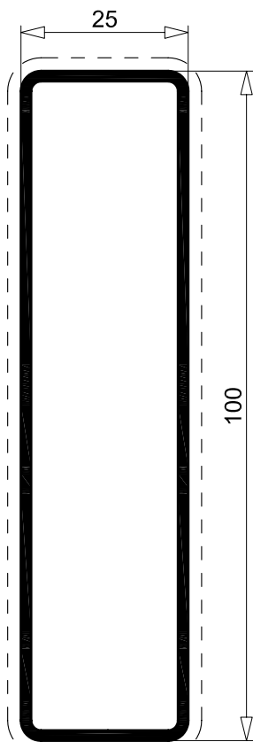
R 3219 0.985 Kg/m sup. in vista 250 mm per. esterno 250 mm
