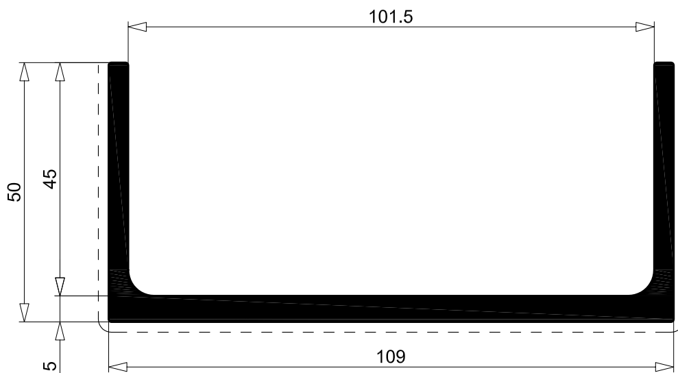
B 1143 2.411 Kg/m sup. in vista 208 mm per. esterno 402 mm
