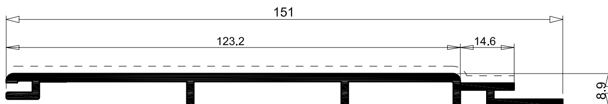
I 3582 1.084 Kg/m sup. in vista 139 mm per. esterno 403 mm
