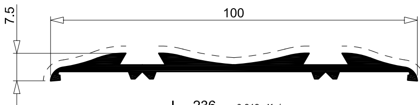
I 236 0.818 Kg/m sup. in vista 88 mm per. esterno 243 mm
