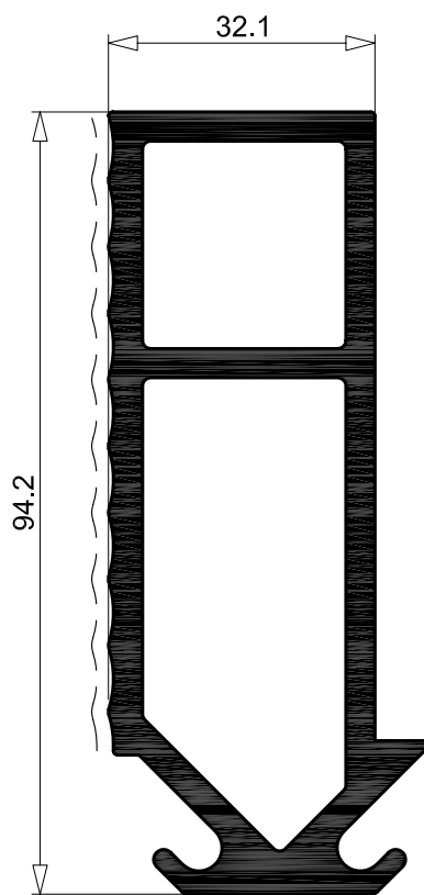
R 10630 2.700 Kg/m sup. in vista 78 mm per. esterno 285 mm
