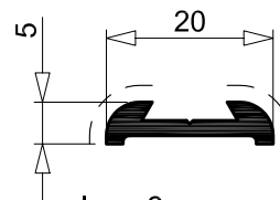
I 8 0.147 Kg/m sup. in vista 18 mm per. esterno 56 mm
