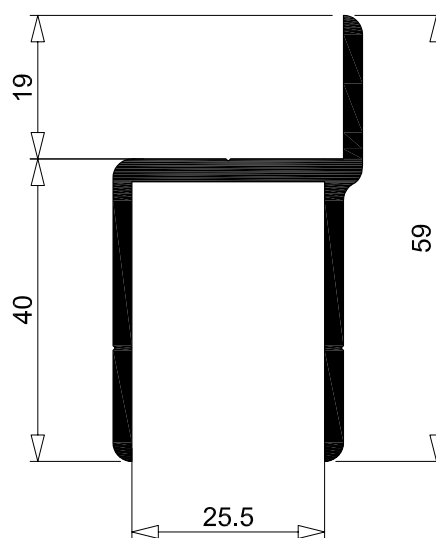
B 327 0.880 Kg/m sup. in vista X mm per. esterno X mm
