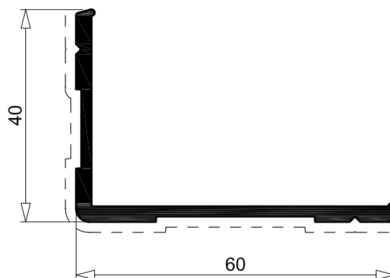
AI 0023 0.626 Kg/m sup. in vista 102 mm per. esterno 204 mm
