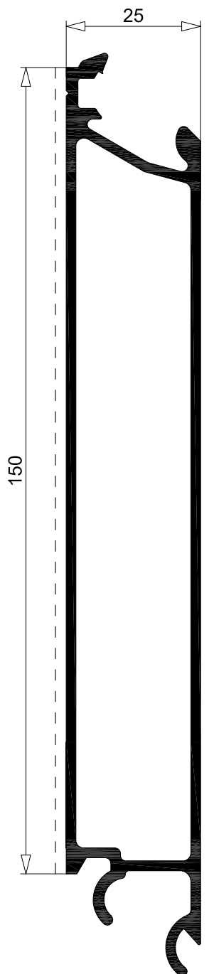
R 7351 1.968 Kg/m sup. in vista 298 mm per. esterno 490 mm
