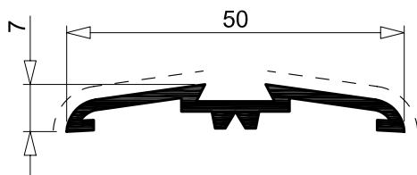
I 272 0.301 Kg/m sup. in vista 46 mm per. esterno 137 mm
