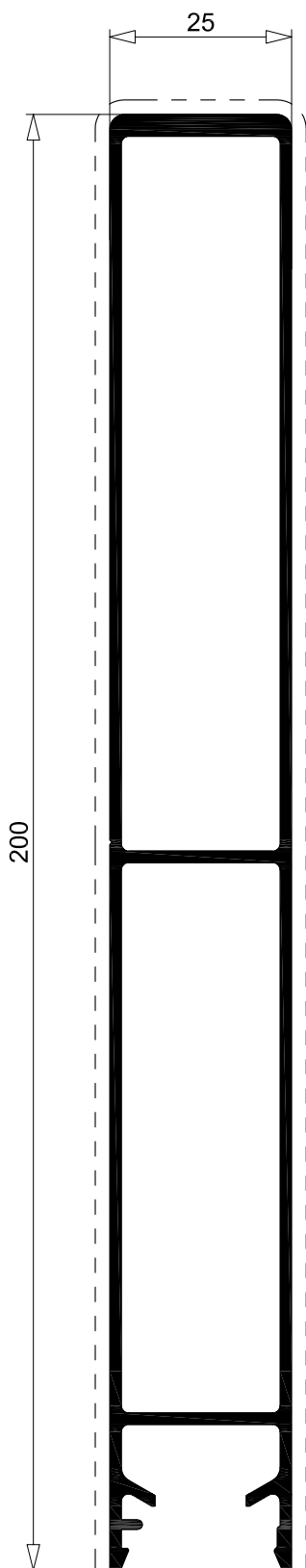
R 3478 2.157 Kg/m sup. in vista 225 mm per. esterno 511 mm
