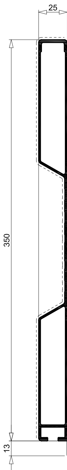
R 7784 3.308 Kg/m sup. in vista 396 mm per. esterno 849 mm
