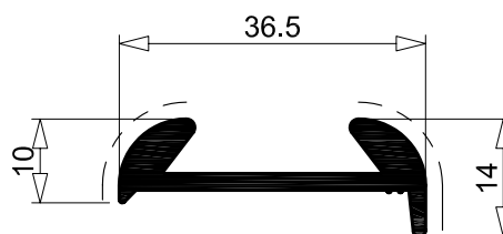
I 5567 0.482 Kg/m sup. in vista 32 mm per. esterno 117 mm
