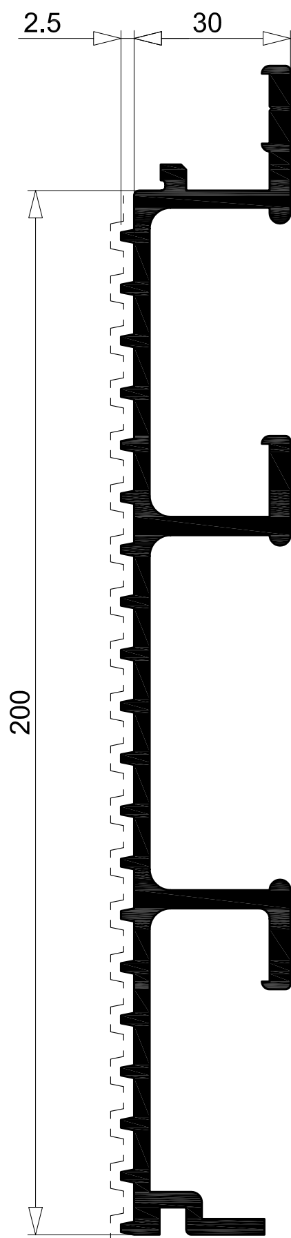
R I 3190 3.664 Kg/m sup. in vista 200 mm per. esterno 831 mm
