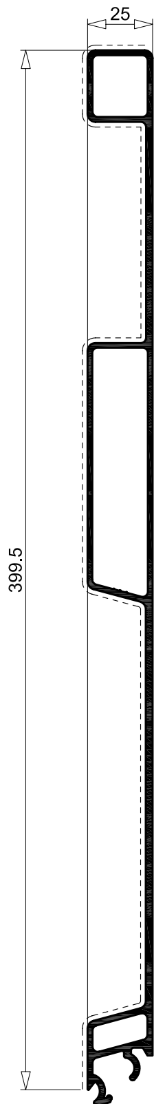
R 8842 3.964 Kg/m sup. in vista 487 mm per. esterno 965 mm
