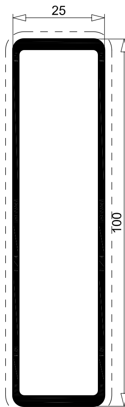
R 3660 1.196 Kg/m sup. in vista 244 mm per. esterno 244 mm
