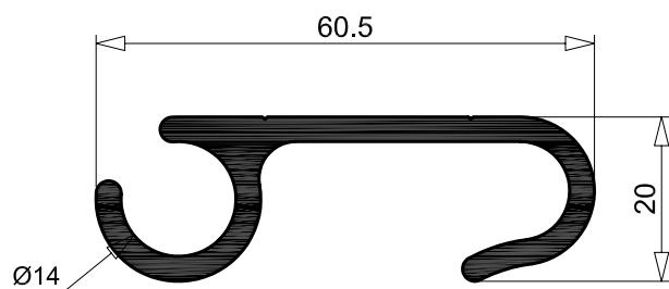
AB 0003 0.924 Kg/m sup. in vista X mm per. esterno 219 mm
