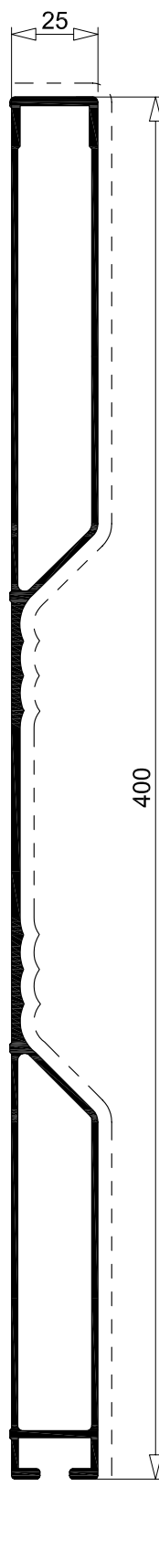
R 5305 4.109 Kg/m sup. in vista 449 mm per. esterno 914 mm
