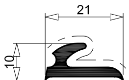
A 34 0.210 Kg/m sup. in vista 36 mm per. esterno 66 mm
