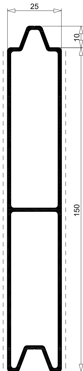
R 7071 1.598 Kg/m sup. in vista 300 mm per. esterno 375 mm
