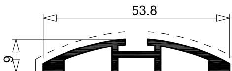
F 552 0.347 Kg/m sup. in vista 50 mm per. esterno 151 mm
