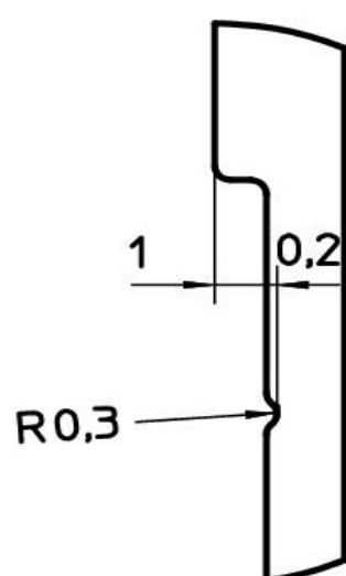
DETAIL A M 5:1
