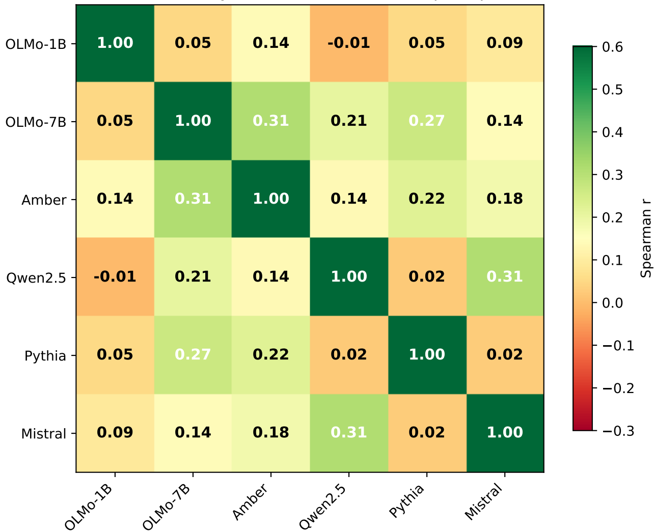
Cross-family alignment correlation (3-token storyline survival across 71 prompts)
