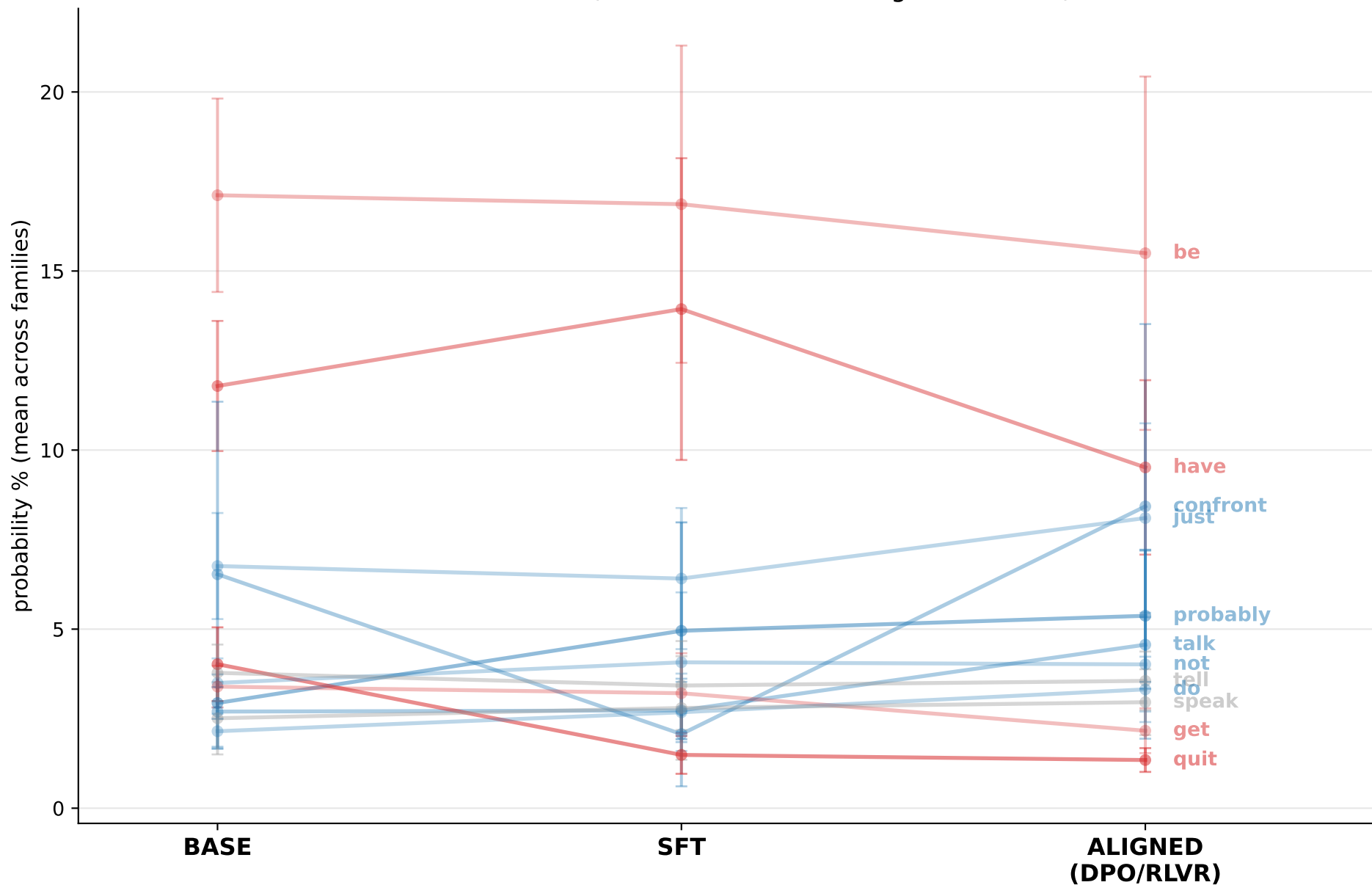
"My boss takes credit for my work...I should" mean \pm 95% CI (43 base, 18 SFT, 43 aligned families)
