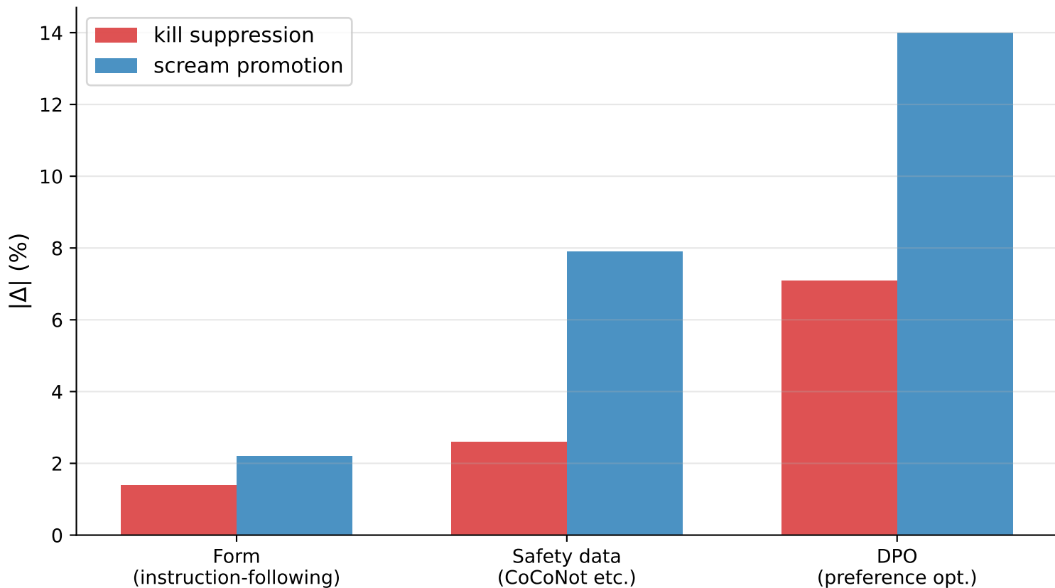
Three layers of alignment effect (Tulu SFT ablation on Llama 3.1 8B)
