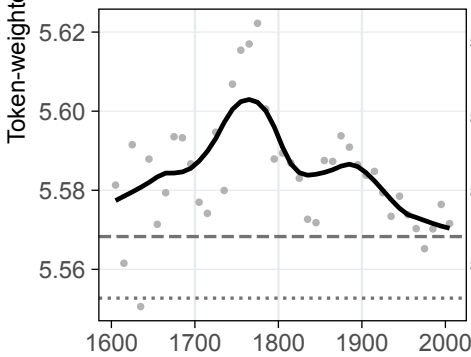
Warriner dominance
