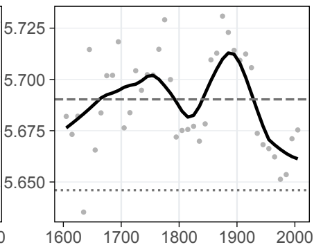
Warriner valence
