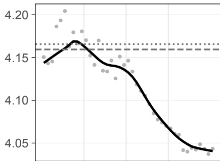
Warriner valence
