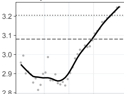
Warriner dominance
