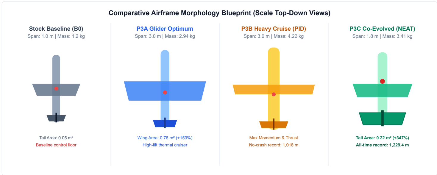
Figure 3.1: Top-Down Scale Blueprints of Evaluated Airframe Morphologies. Notice the dramatic expansion of tail surfaces in P3C relative to Stock (B0), P3A, and P3B.
