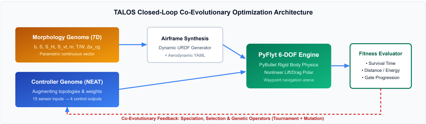
Figure 1.1: Complete Project TALOS Co-Evolutionary Closed-Loop Architecture, illustrating parametric URDF generation, parallel 6-DOF simulation, and tournament-based genetic optimization.
