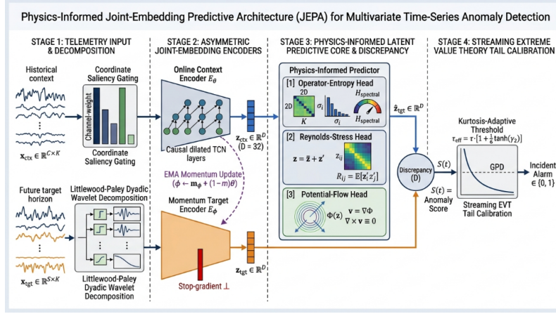
Fig. 1. JEPA telemetry-monitoring architecture: context and suspect windows are encoded into z_{ctx} , z_{tgt} and compared in latent space (avoiding observation-space false-alarm flooding), under three candidate physical regularizers (Koopman spectral entropy, covariance closure, potential flow) with held-out SPOT calibration.
