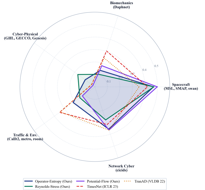
Fig. 3. PR-AUC radar comparison across five specialized physical domains: Spacecraft Telemetry (MSL, SMAP, swan), Biomechanics (Daphnet), Cyber-Physical Systems (GHL, GECCO, Genesis), Traffic & Environmental (Callt2, metro, room-occupancy), and Network Cyber (CICIDS). The physics-inspired triad provides broad multi-domain coverage.
