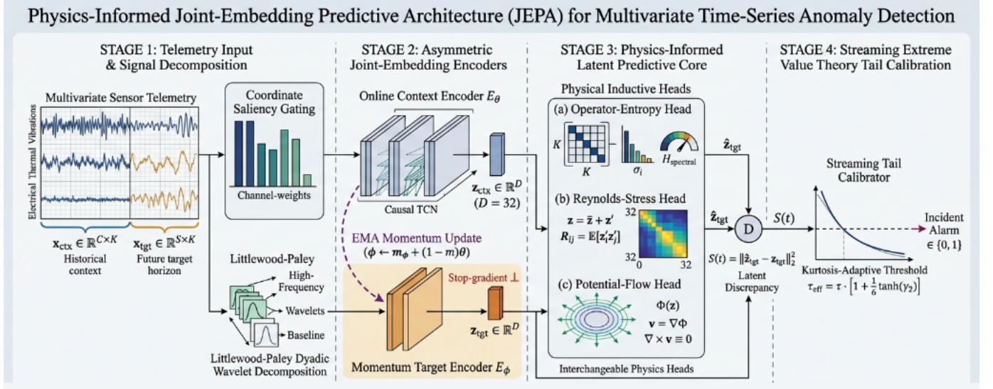
Fig. 1. Architectural overview of the proposed Physics-Informed Joint-Embedding Predictive Architecture (JEPA) framework. The historical context window \mathbf{x}_{\text{ctx}} and suspect target window \mathbf{x}_{\text{tgt}} are projected through multi-scale dyadic TCN encoders into latent representations \mathbf{z}_{\text{ctx}} and \mathbf{z}_{\text{tgt}} . Rather than reconstructing raw observation-space waveforms (which causes false alarm flooding under ambient sensor jitter), the predictive core operates strictly in latent representation space, governed by three complementary physical inductive biases: Koopman operator spectral entropy, hydrodynamic Reynolds stress transport, and conservative potential flow field theory. Prediction discrepancy is calibrated online via streaming Extreme Value Theory (SPOT).
