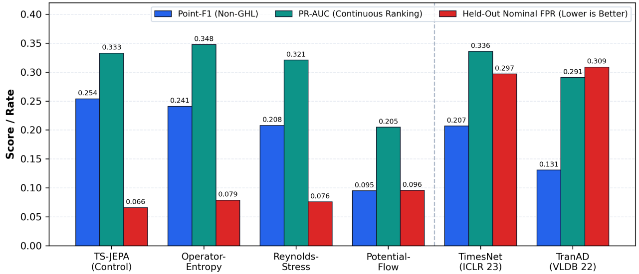
Held-Out Calibration Benchmark (33 Streams, Non-GHL Stream-Macro Means)
