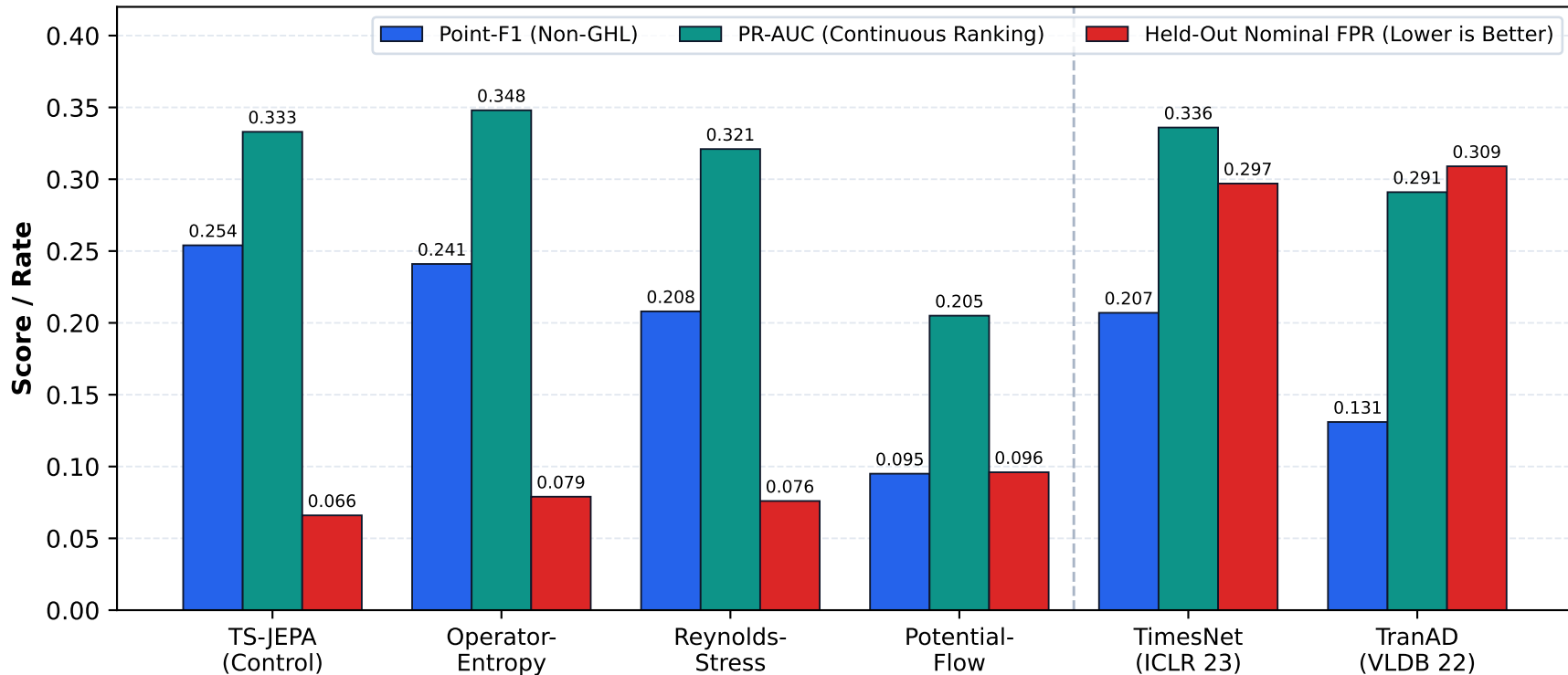
Held-Out Calibration Benchmark (33 Streams, Non-GHL Stream-Macro Means)
