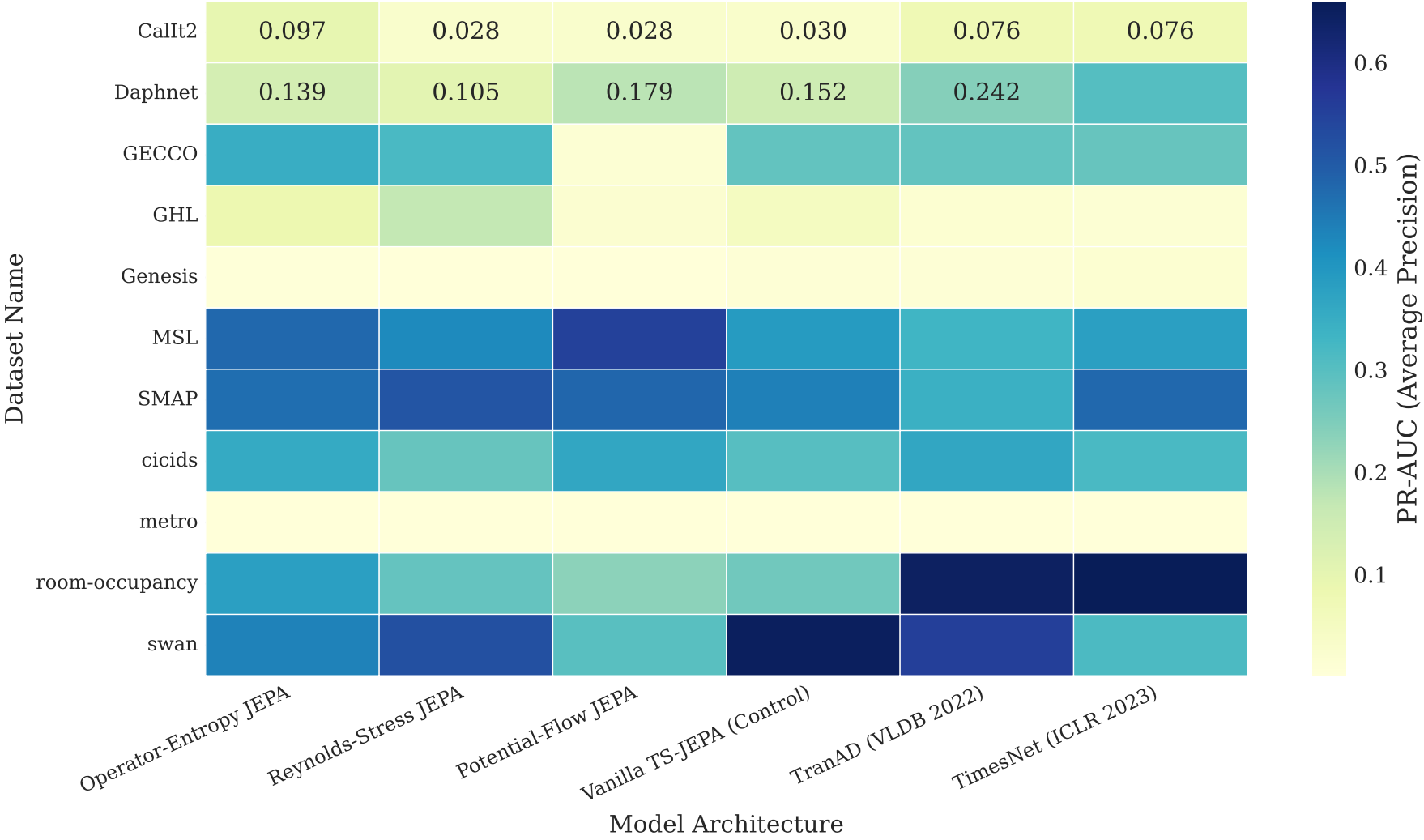
Threshold-Independent PR-AUC Matrix Across Core Telemetry Datasets
