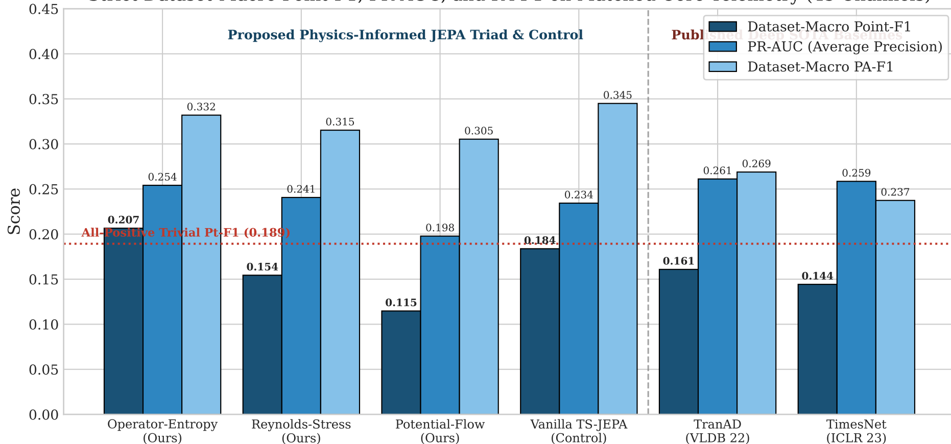
Strict Dataset-Macro Point-F1, PR-AUC, and PA-F1 on Matched Core Telemetry (45 Channels)
