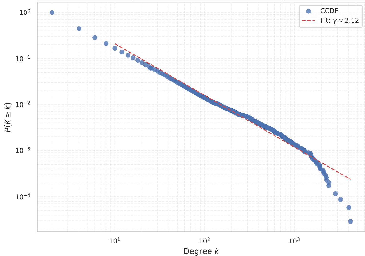
CCDF Degree Distribution: Abe-Suzuki Italy 5 km
