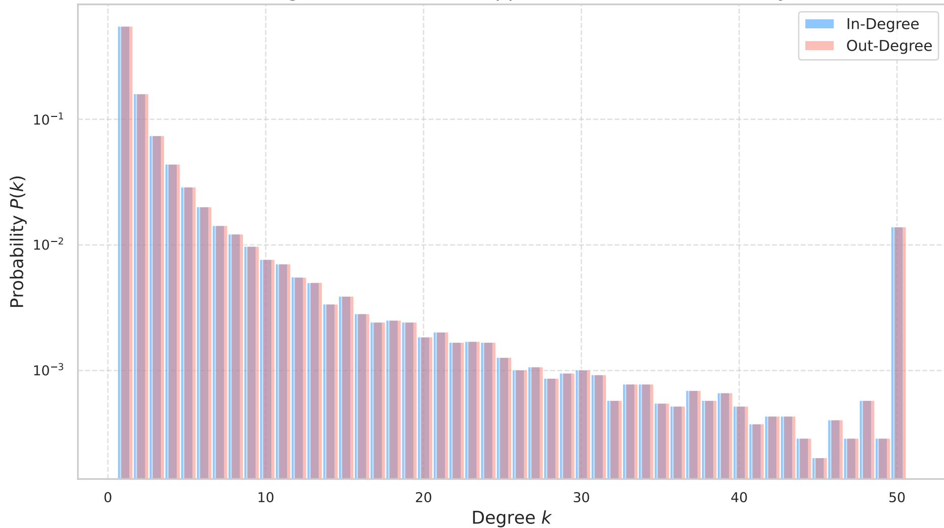
In vs Out Degree Distribution (capped at 50): Abe-Suzuki Italy (5 km)
