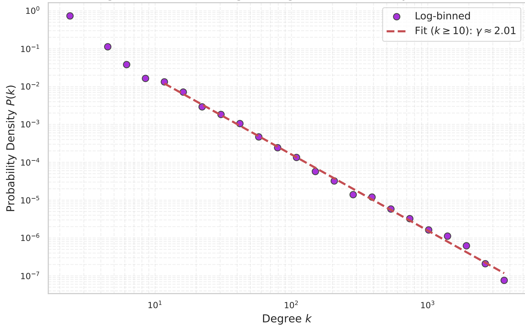
Degree Distribution (Log-Binning): Abe-Suzuki Italy (5x5x5 km)
