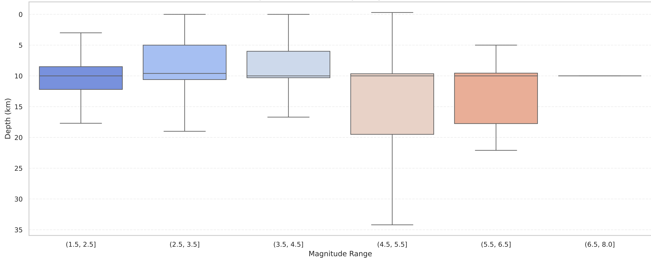
Depth Distribution by Magnitude Bin
