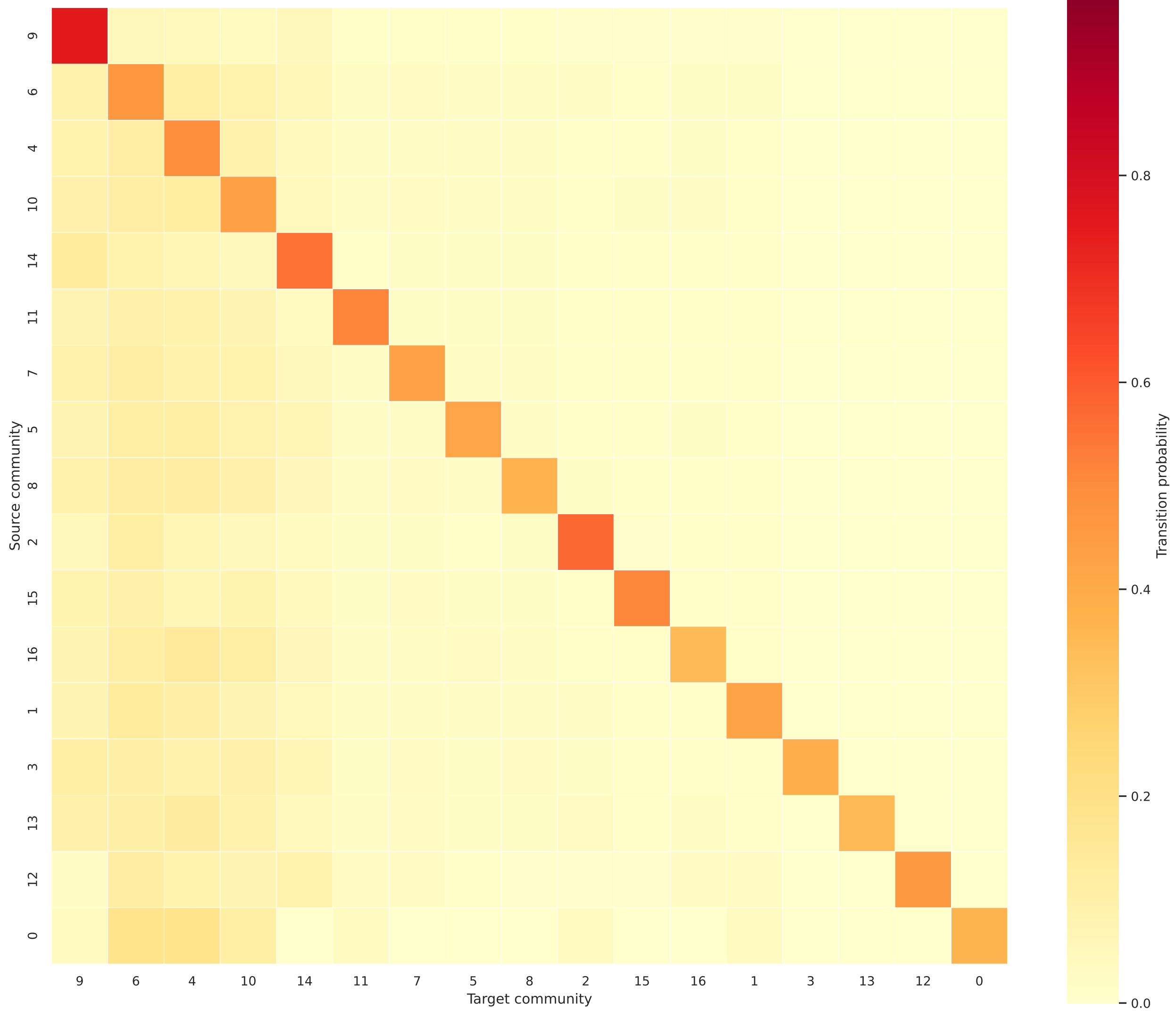
Community Markov Flow — Abe-Suzuki Italy (10 km)
