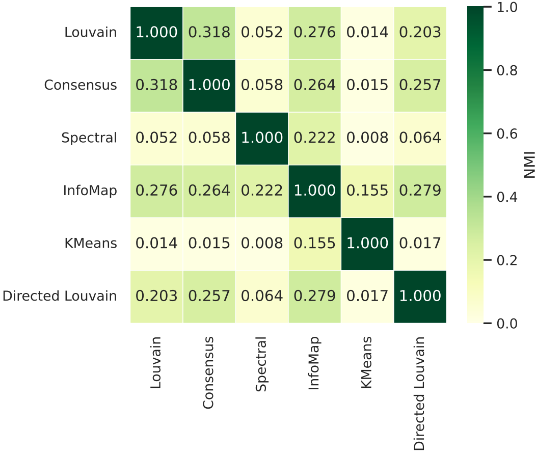
Community Method Agreement (NMI): Abe-Suzuki Italy — directed vs undirected
