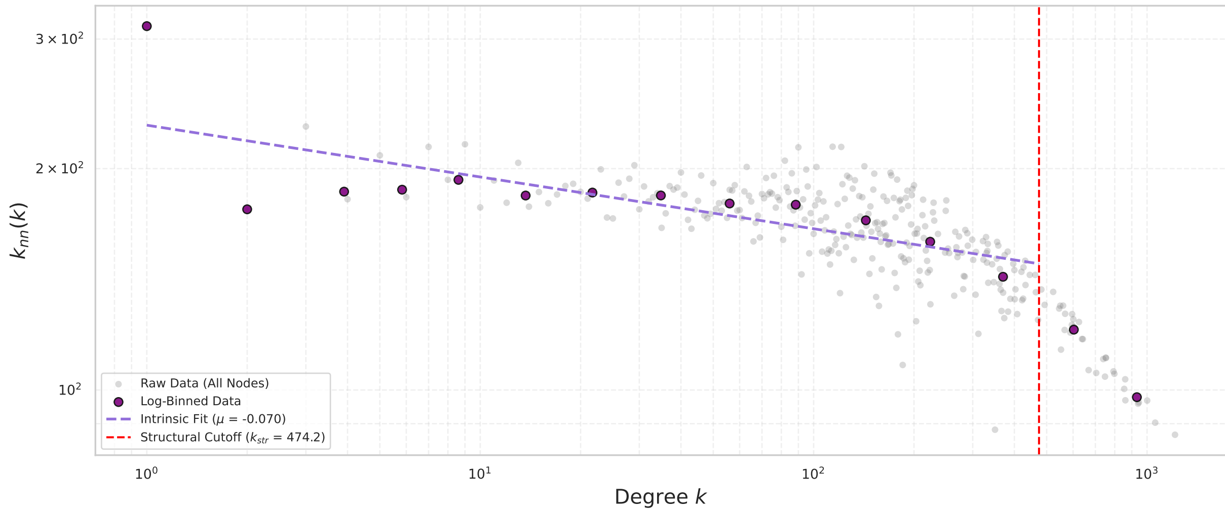
Assortativity Fit
