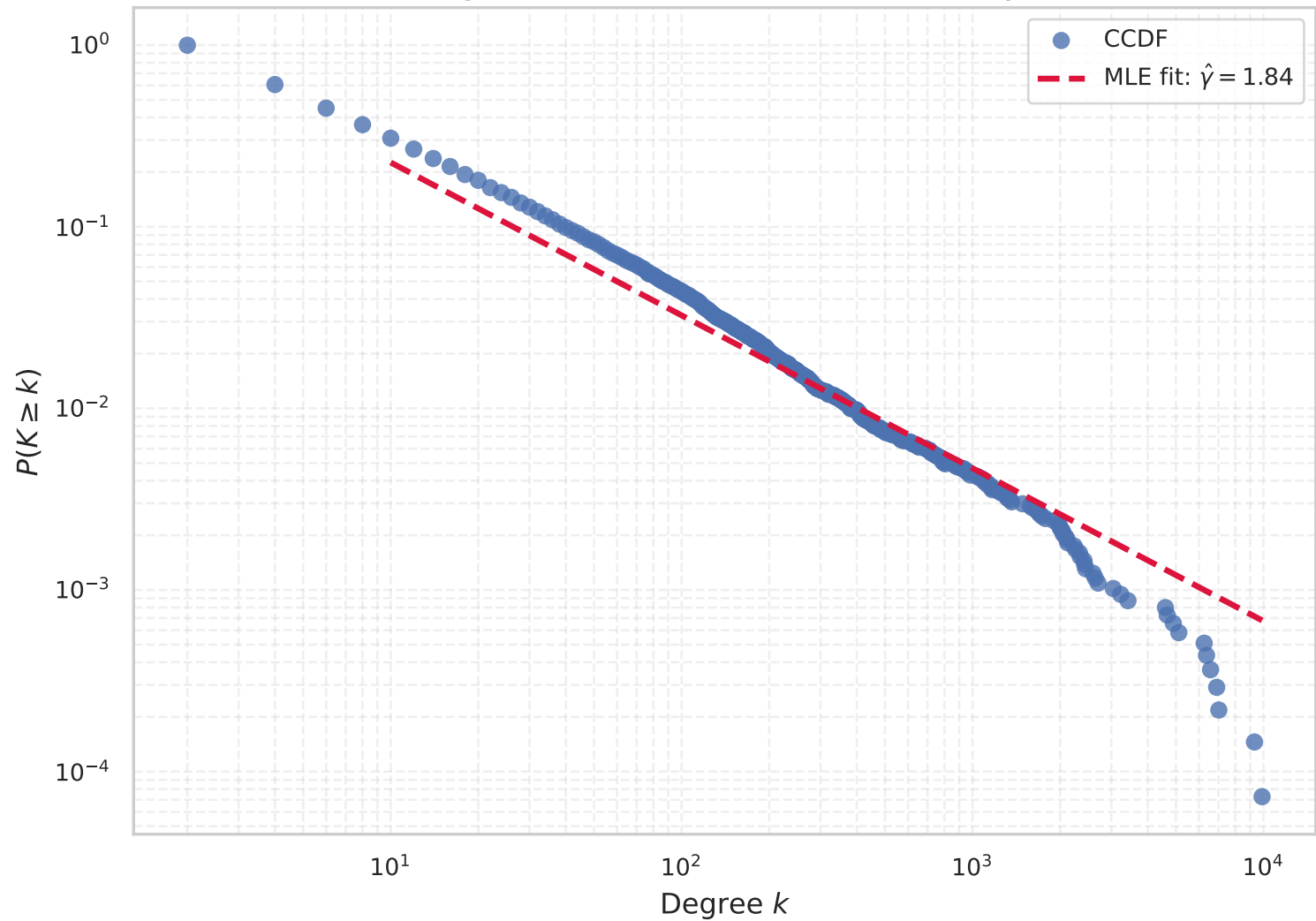
CCDF Degree Distribution: Abe-Suzuki Italy 10 km
