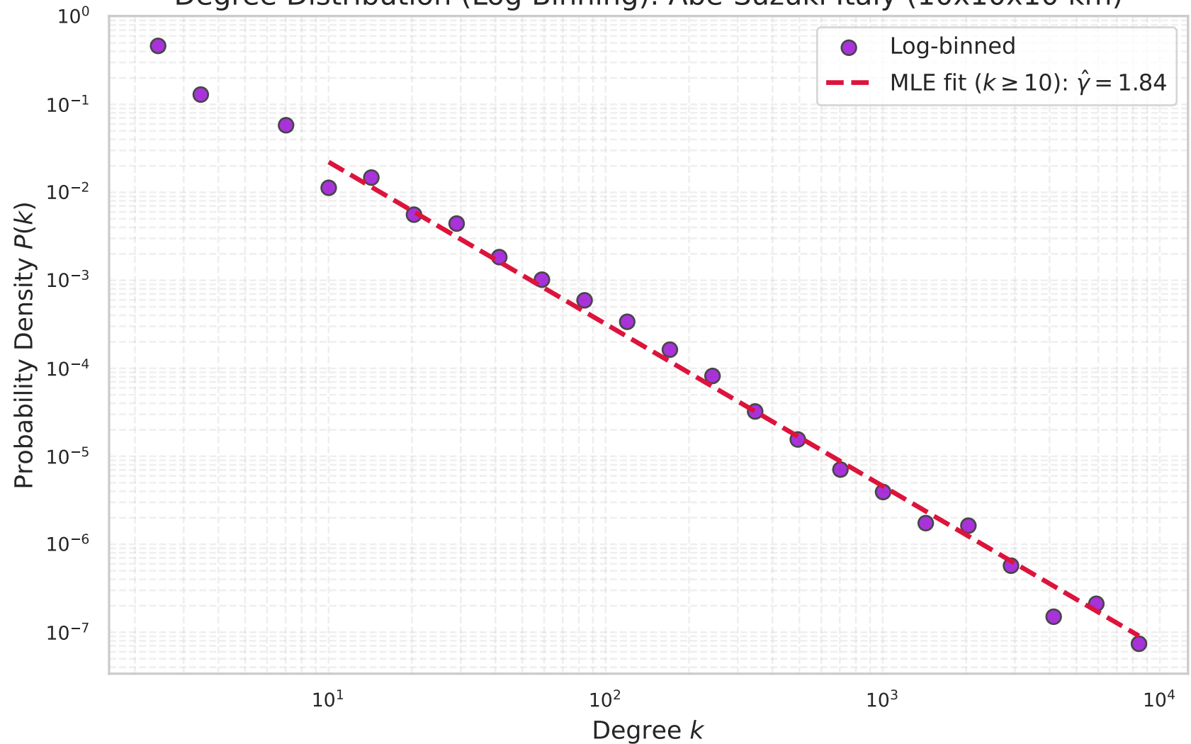
Degree Distribution (Log-Binning): Abe-Suzuki Italy (10x10x10 km)
