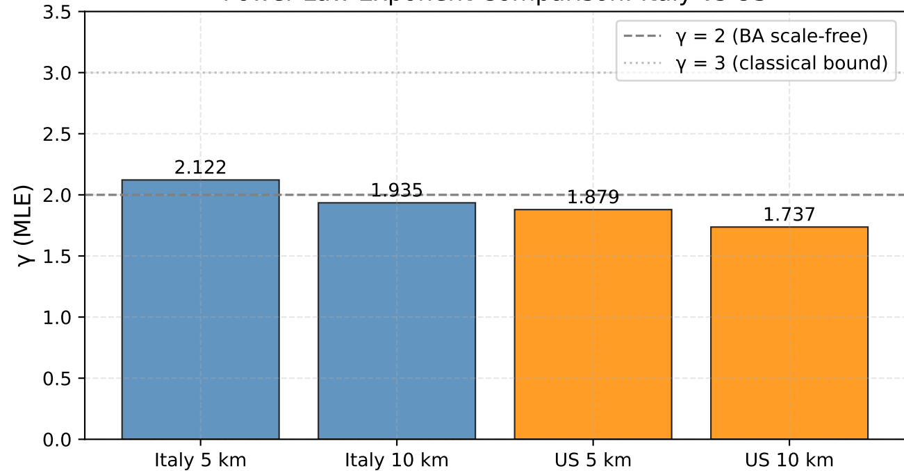
Power-Law Exponent Comparison: Italy vs US
