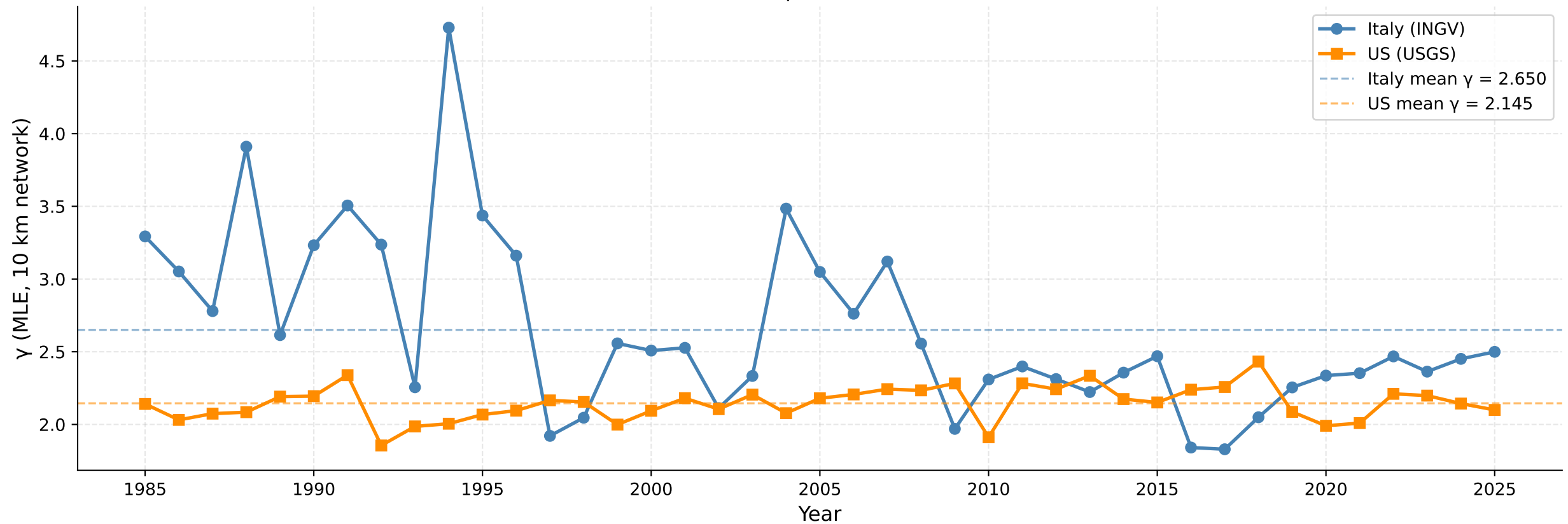
Temporal Evolution of Power-Law Exponent \gamma(t) : Italy vs US (Abe-Suzuki 2004 claim: \gamma should be constant over time)
