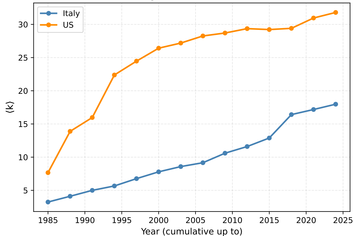
Mean Degree \langle k \rangle — should stabilise
