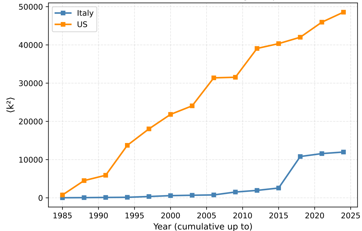
Second Moment \langle k^2 \rangle — diverges if \gamma < 3
