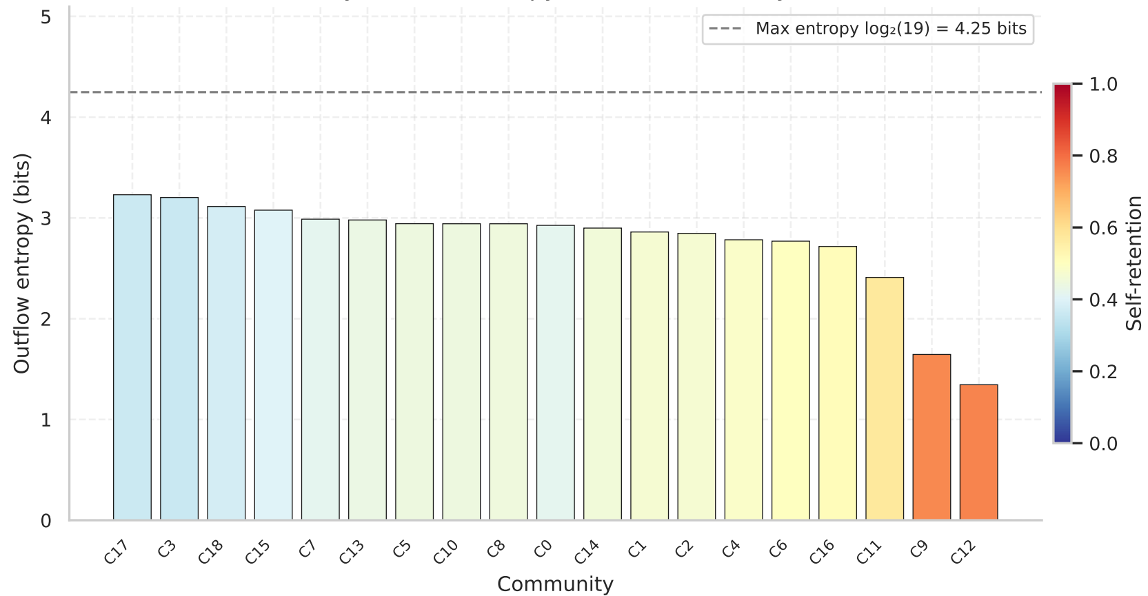
Community Outflow Entropy — Abe-Suzuki Italy (10 km)
