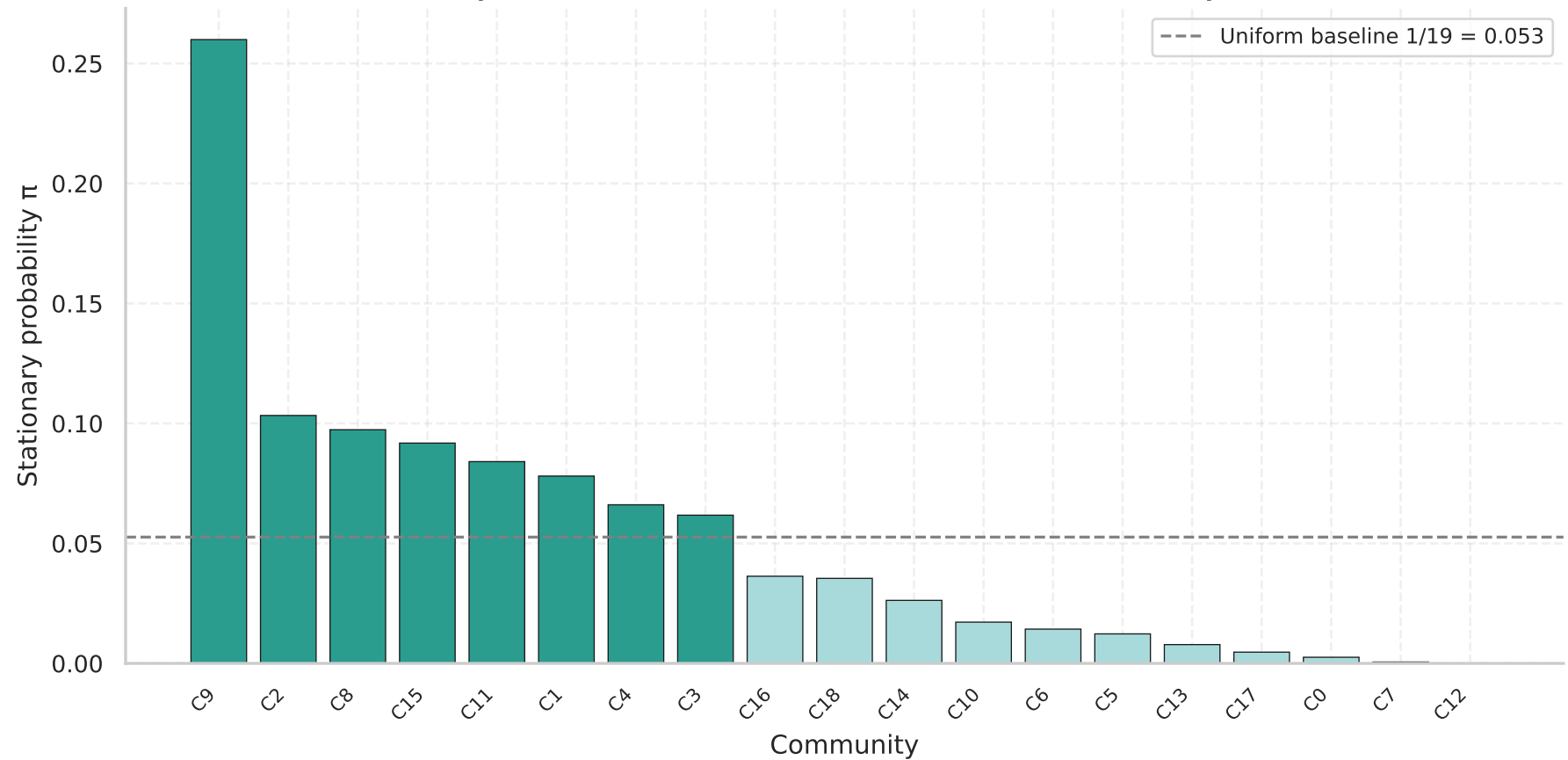
Stationary Distribution of Seismic Flow — Abe-Suzuki Italy (10 km)
