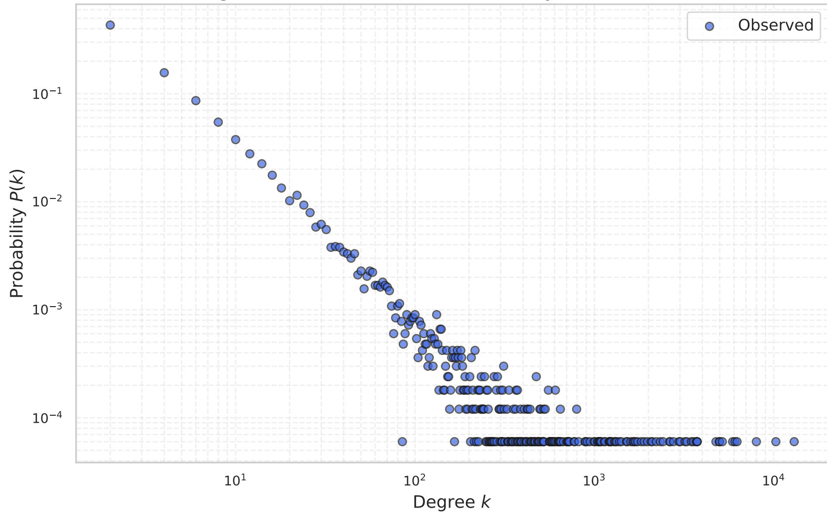
Degree Distribution: Abe-Suzuki Italy (10x10x10 km)
