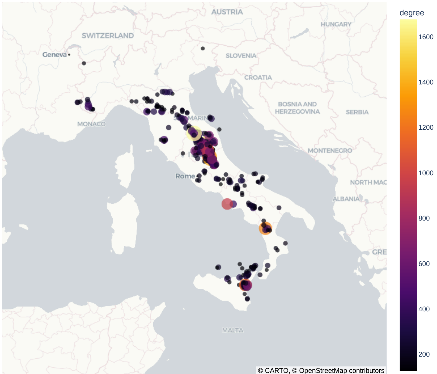
Abe-Suzuki Network Hubs: Top 2% Most Active Seismic Cells — Italy (10x10x10 km)
