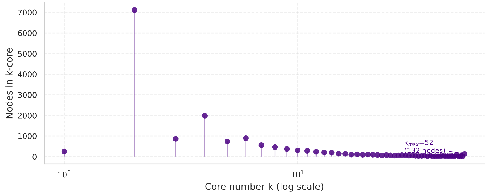
k-core Size Distribution — Italy (10 km)
