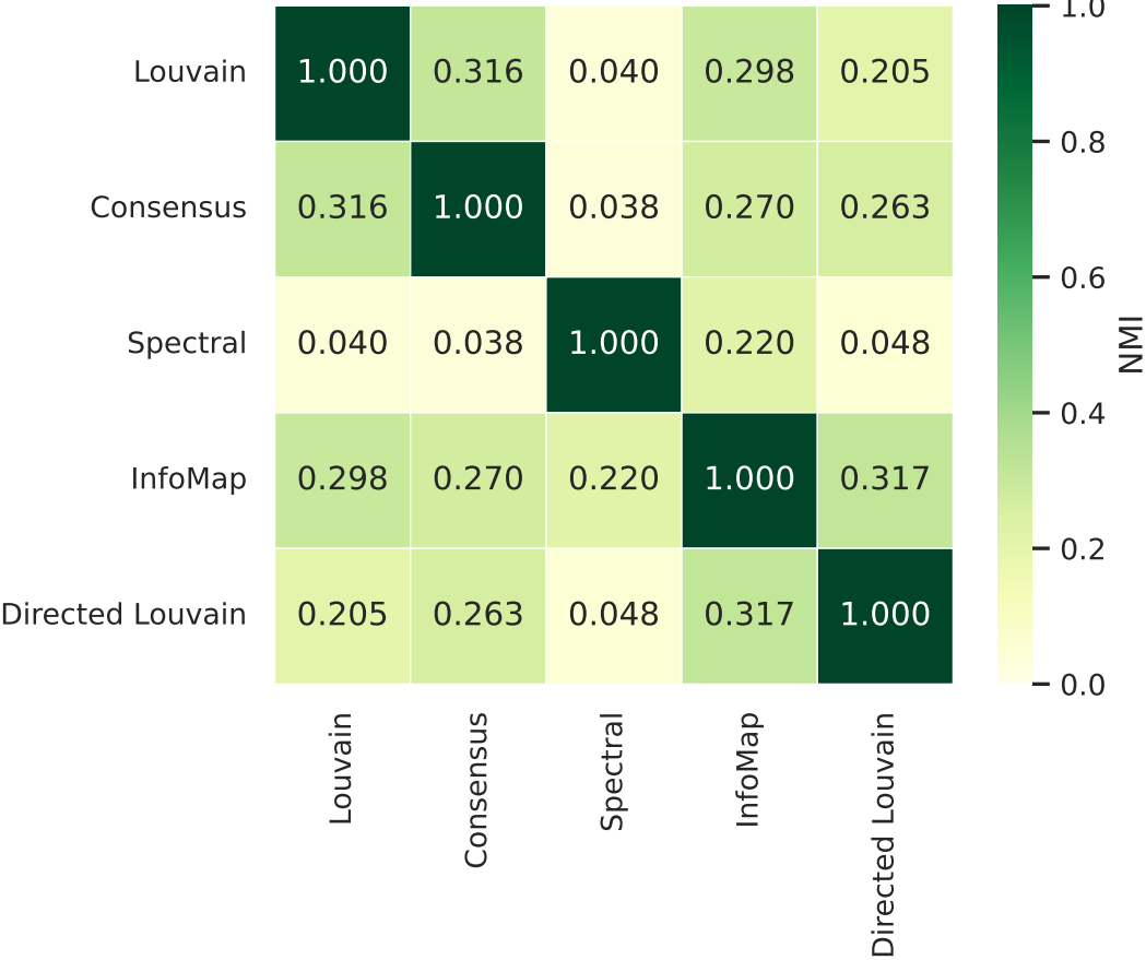
Community Method Agreement (NMI): Abe-Suzuki Italy — directed vs undirected
