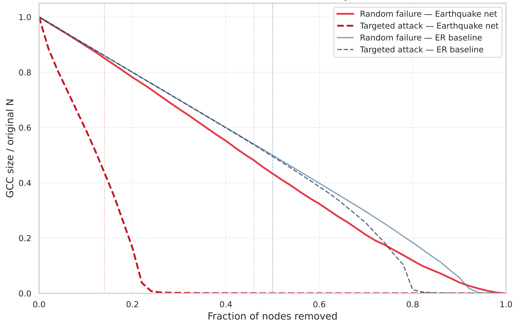
Network Robustness: Abe-Suzuki Italy (10 km)
