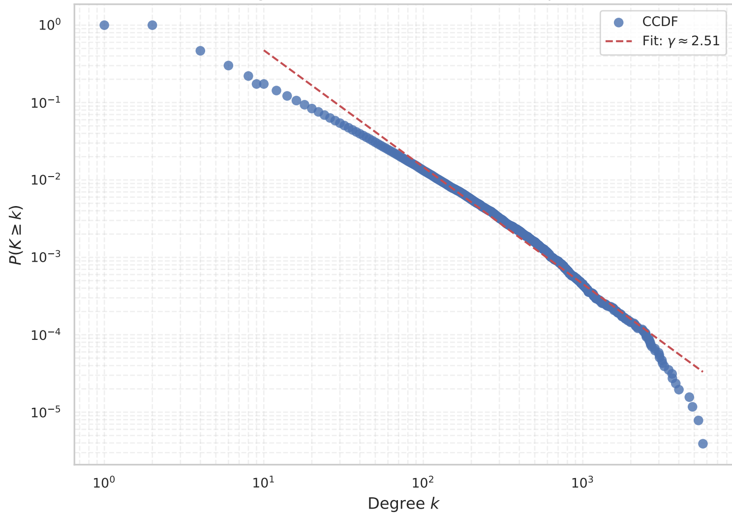
CCDF Degree Distribution: Abe-Suzuki Japan 5 km
