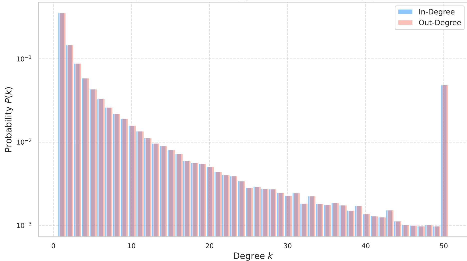
In vs Out Degree Distribution (capped at 50): Abe-Suzuki Japan (10 km)
