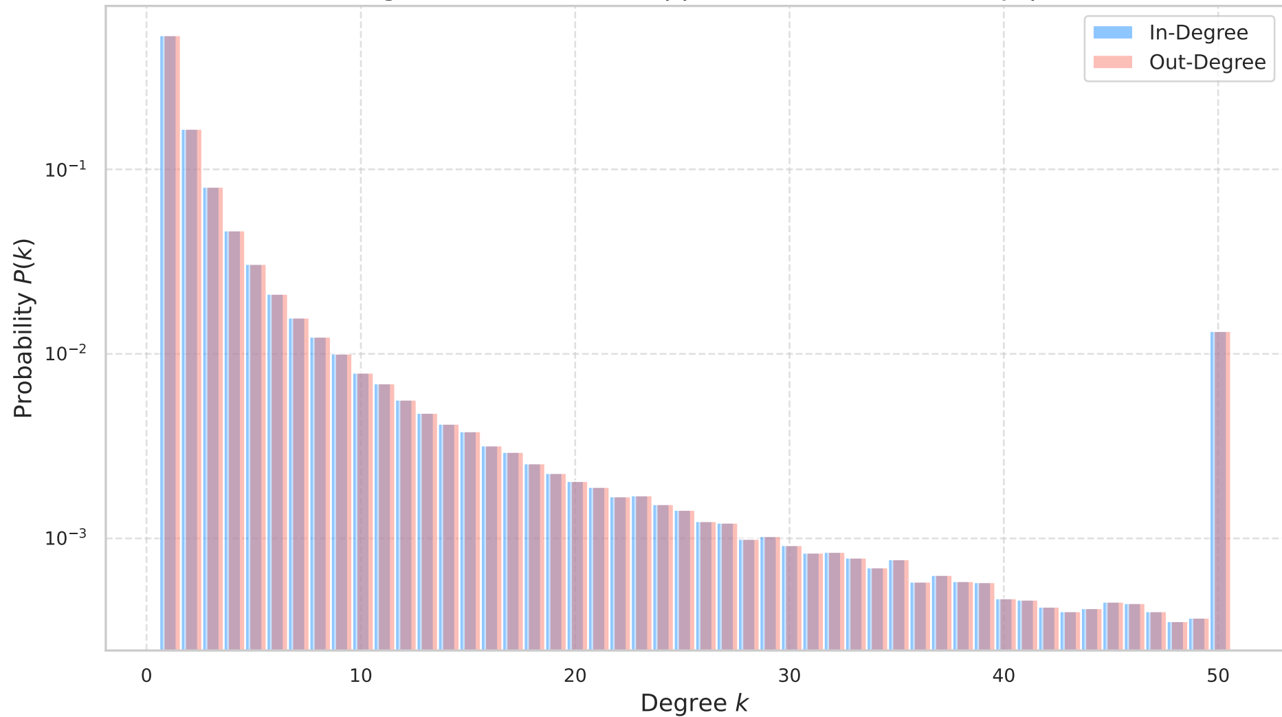
In vs Out Degree Distribution (capped at 50): Abe-Suzuki Japan (5 km)
