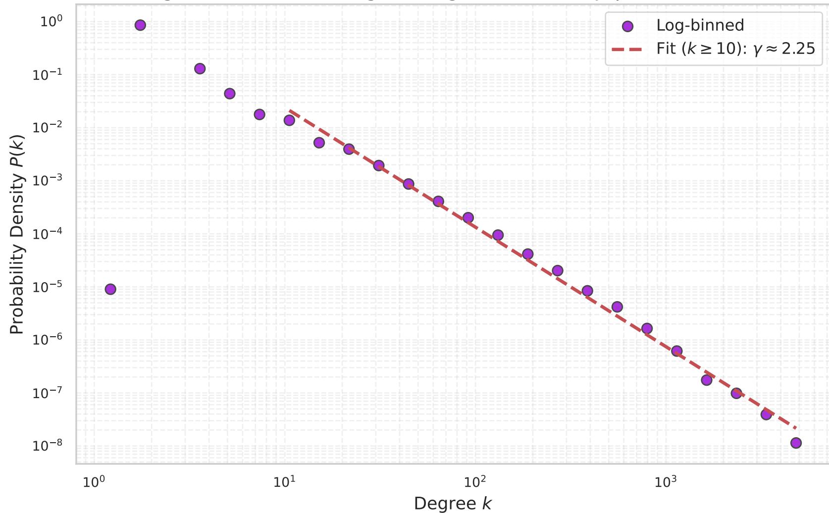
Degree Distribution (Log-Binning): Abe-Suzuki Japan (5x5x5 km)
